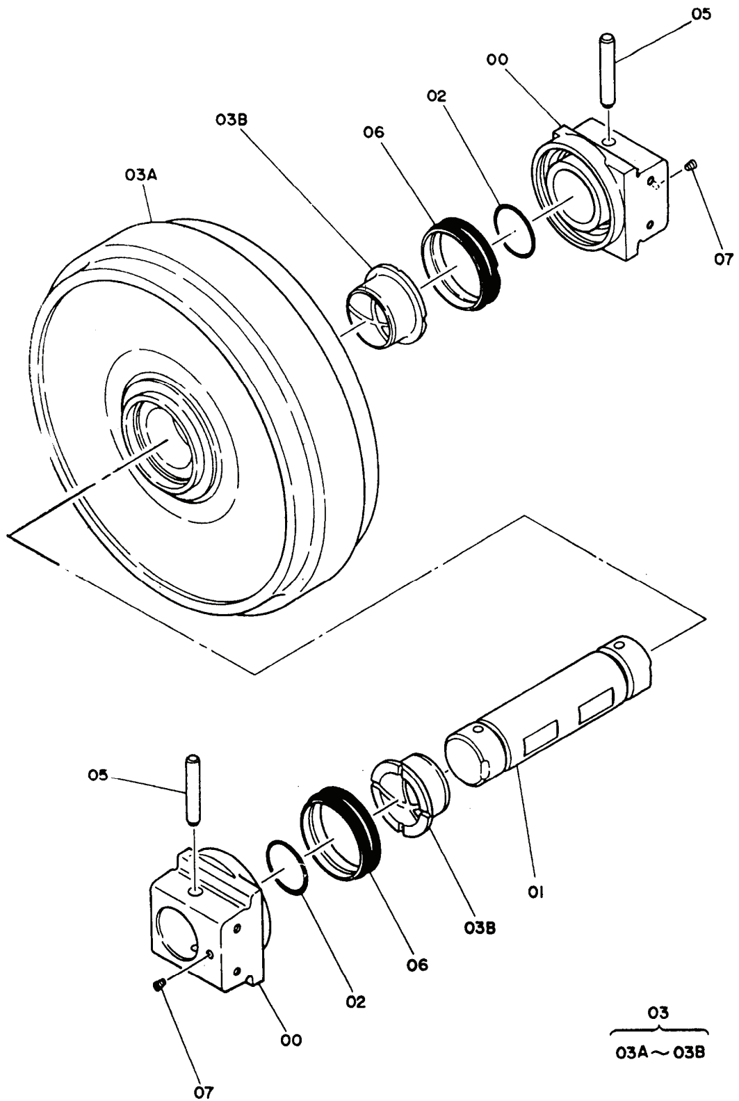
FRONT IDLER
